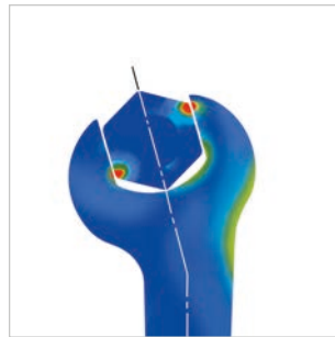
2 Load zones in spanners by STAHLWILLE
