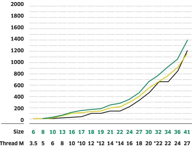
N-m Test results STAHLWILLE combination spanners No 13 (open-jaw)
