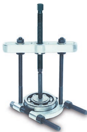
Separating fixture in use for removing ball bearings
