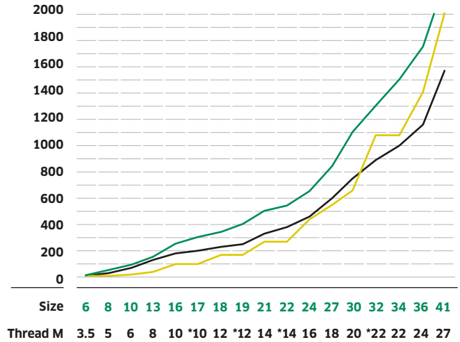
N-m Test results STAHLWILLE combination spanners No 13 (ring)
