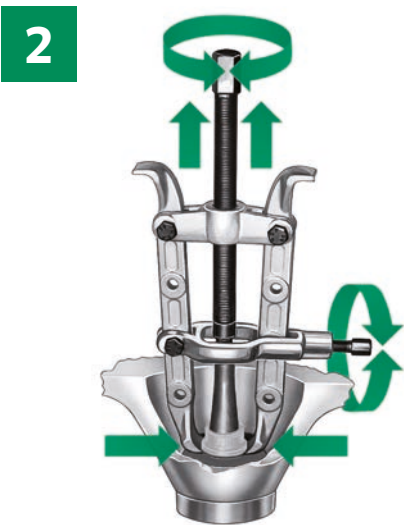
2 How a two-armed puller works
